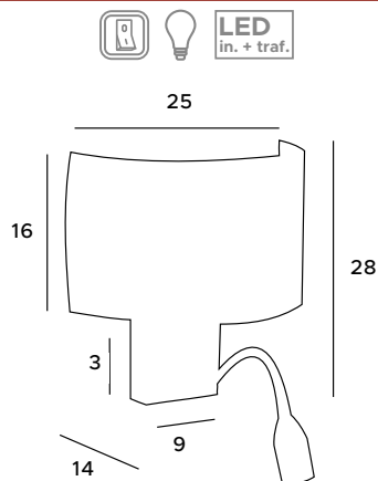
W0049 1 x 40W 230V + 2W LED chrom, biały abażur chrome, white shade metal, tkanina metal, fabric
