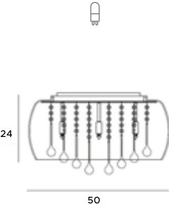
C0076-06X 6x40W G9 230V chrom chrome szkło lustrzane, metal mirror glass, metal
