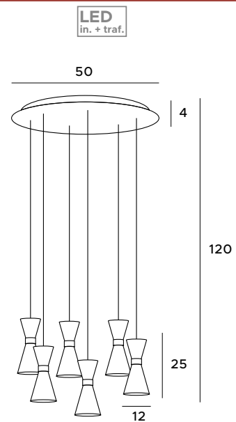
P0331 6x5W LED 1800lm 3000K czarny, złoto black, gold metal metal
