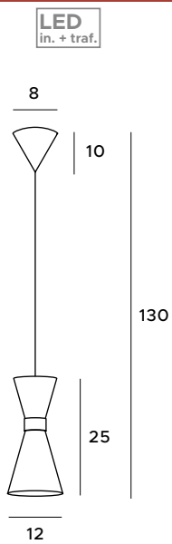
P0330 1x5W LED 300lm 3000K czarny, złoto black, gold metal metal
