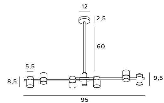
P0409 max 6 x GU10 5W LED 230V złote, czarne gold, black metal metal
