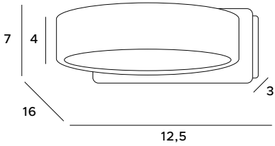
W0167 1x4,5W LED 310lm 3000K czarne, złote black, gold aluminium aluminium LED in. + traf.
